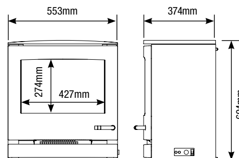
YM-681-093 CL8 Electric Stove Approx. Weight: 44Kg
