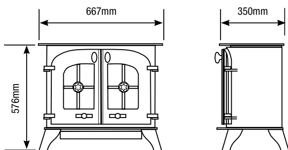
YM-E5201FL Dartmoor 1 Door - flat top Approx. Weight: 75Kg YM-E5202FL Dartmoor 2 Door - flat top Options YM-A9904 Brass handle (single door only)
