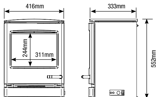
YM-681-048 CL5 Electric Stove Approx. Weight: 47Kg
