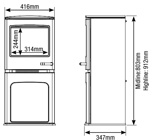
YM-681-003 CL5 Electric Midline Approx. Weight: 56kg YM-681-016 CL5 Electric Highline Approx. Weight: 59kg
