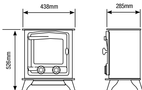
YM-E9001FL Exmoor - flat top Approx. Weight: 47Kg Options YM-A9904 Brass handle
