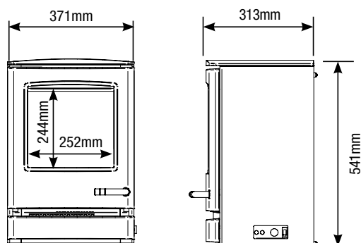
YM-681-021 CL3 Electric Stove Approx. Weight: 40Kg
